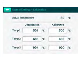
Precision temperature control with a 3-point calibration process
