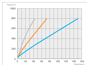
Temperature ramp control (Fastest, 5^{\circ}\text{C}/\text{min} , 10^{\circ}\text{C}/\text{min} ) at the set temperature of 800^{\circ}\text{C} .
