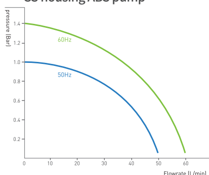
SS housing ABS pump
